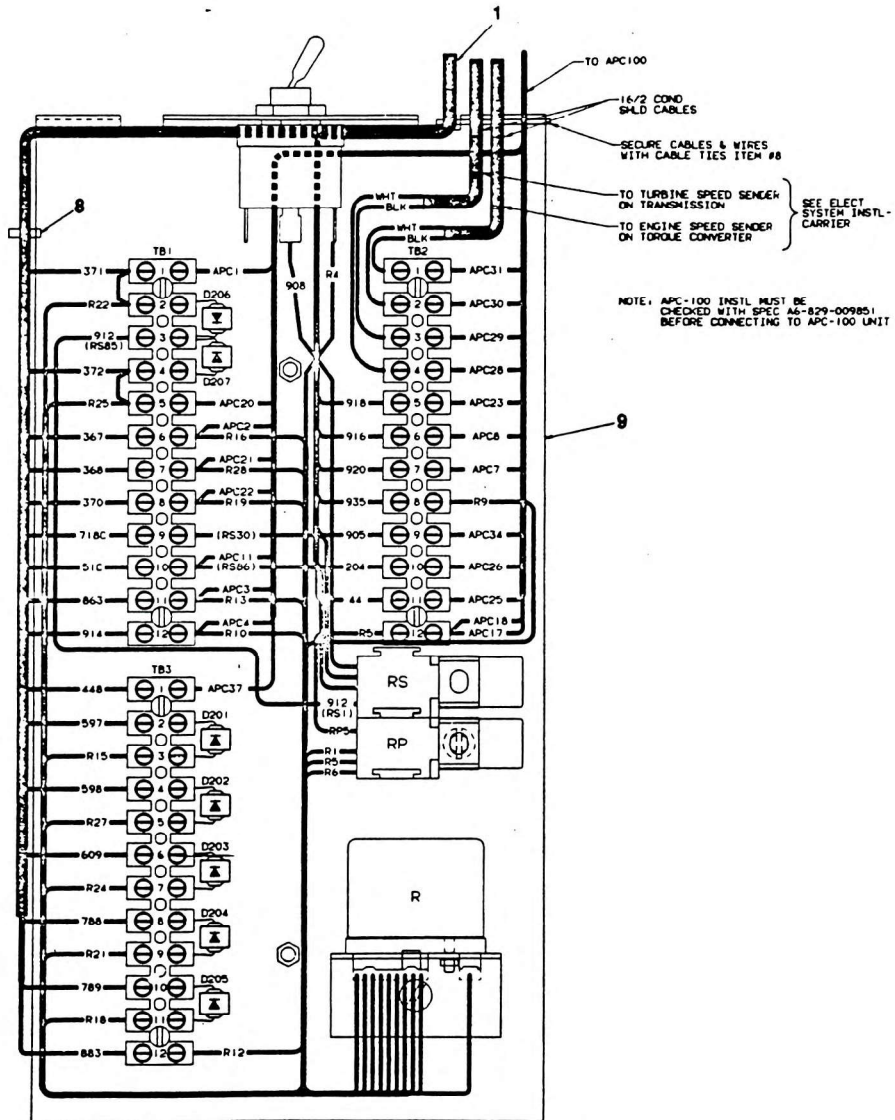
VIEW R APC100 WIRING
